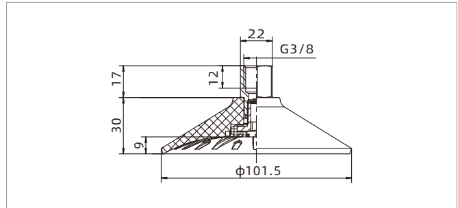
SDM100U-G3F
