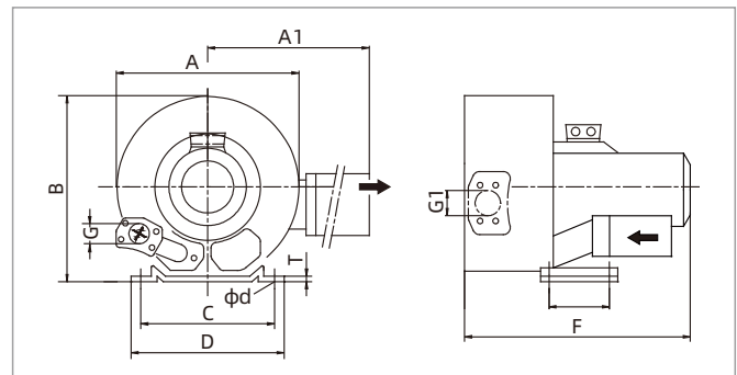
APB-720
