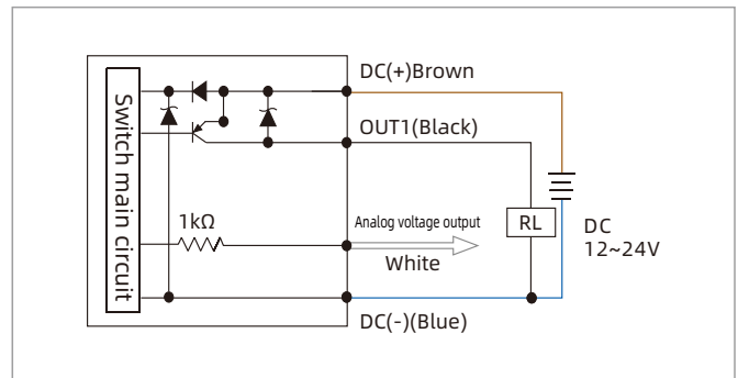
ZPDT-CPV-R1M 1PNP+Analog voltage output(1-5V)
