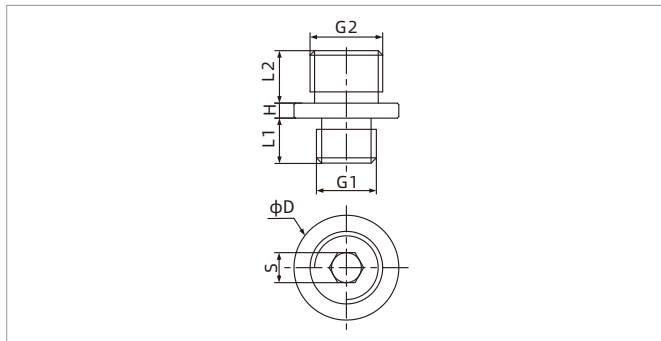
Different diameter male-male thread
