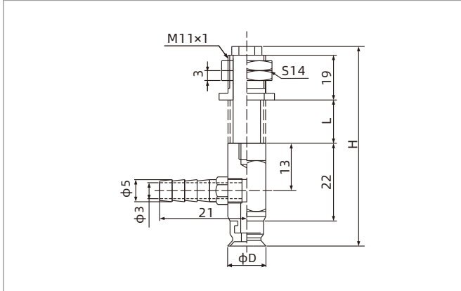
SPF10-20 Lateral-Pagoda fitting
