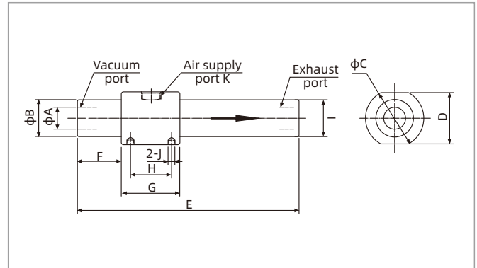
ACPF(Other sizes)
