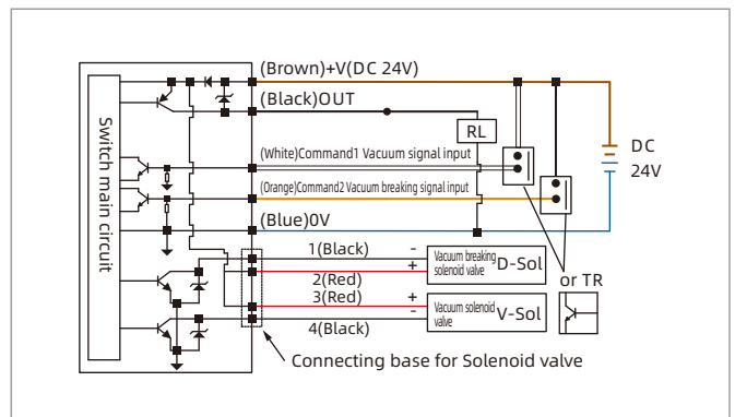
ZPDC-PE(PK/PEO)PNP output
