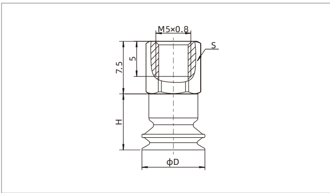
SP3B4-16 F - Female thread connection
