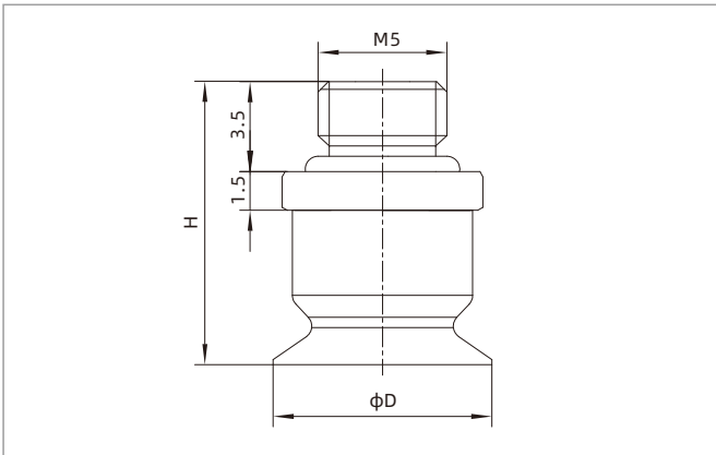
SPHC□CH-M5M
