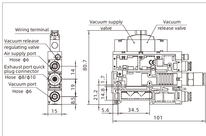
AZK-□-08(10) Single body exhaust port quick plug connector
