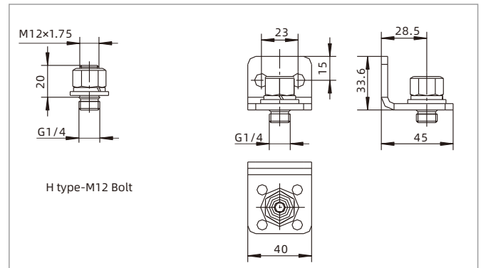
Type H - M12 Bolt
