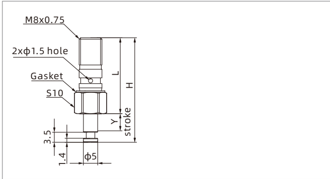
PSPS-I6D5-I8
