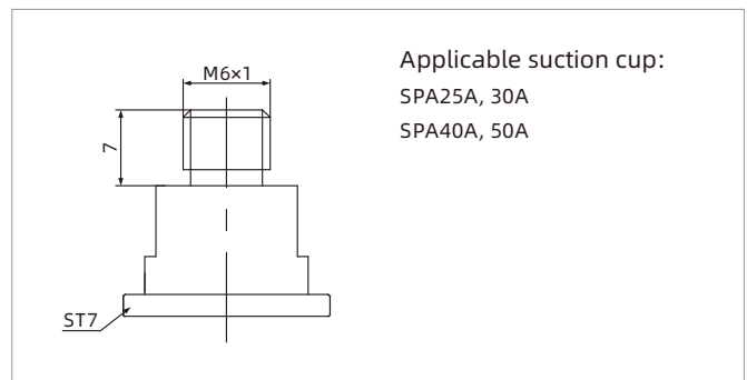
PJS-M6M-ST7
