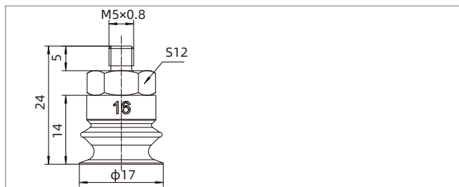
SBT16-M5M
