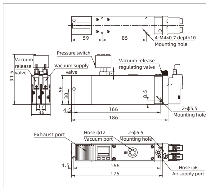
AZL112-A-DCN AZL112-A-DCP
