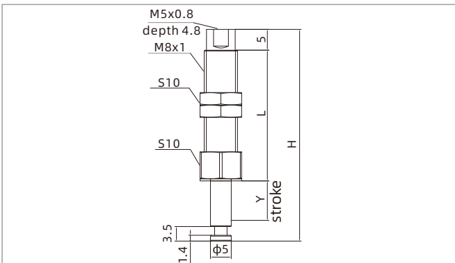
PSPS-I□D5-M8
