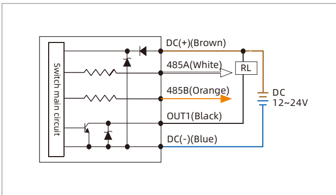
ZPDC-NR 1NPN+1 set Rs485
