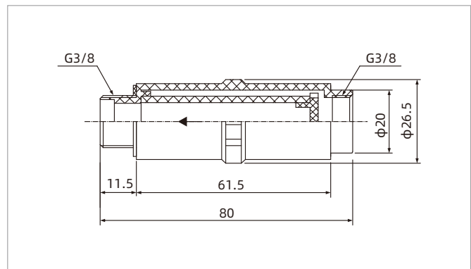
ZFL10
