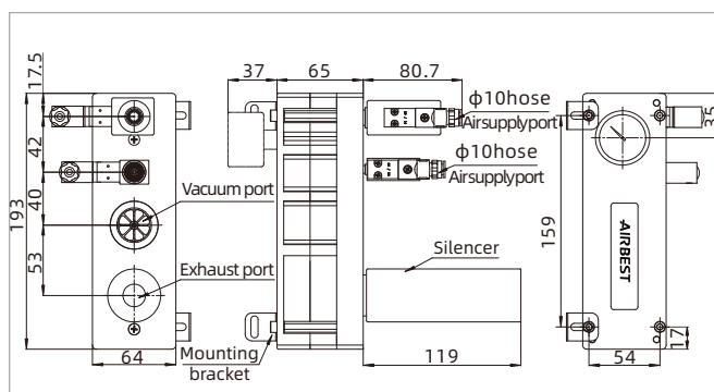
AM/AL75-100-AD/E-PVD
