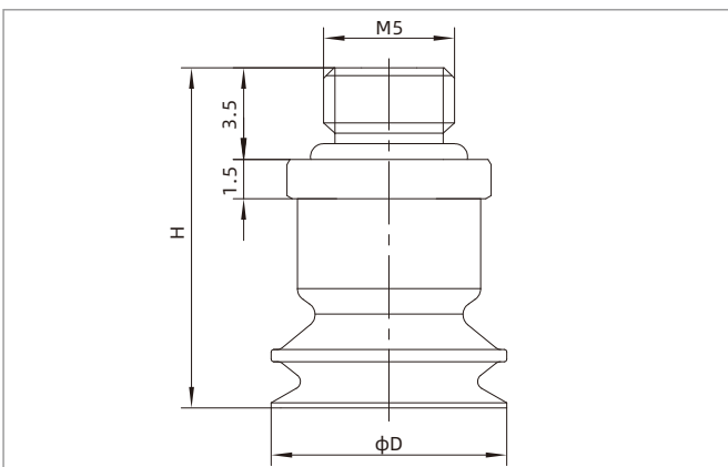
SPHB□CH-M5M
