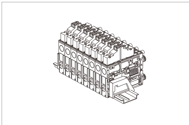
Combined type with guide rail
