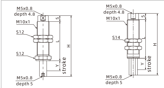
PPSP-□M5F-M10
